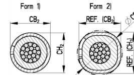
Insulation Crimp Iso Crimp
