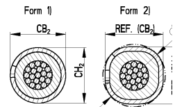
Insulation Crimp Iso Crimp
