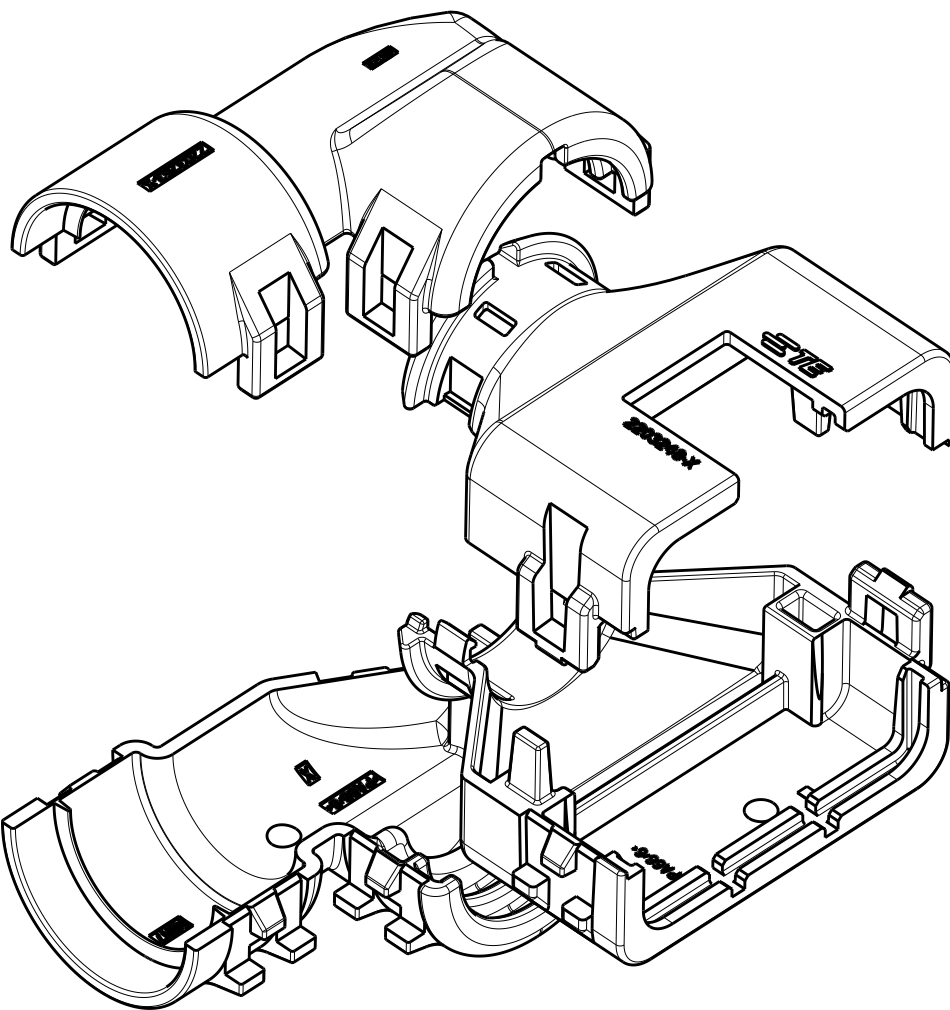
2302495-2 EXPLODED ISOMETRIC VIEW SHOWN 2 3
