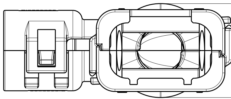
2302491-2 ASSEMBLED VIEW SHOWN DIMENSIONS SHOWN FOR 2302491-2 ONLY
