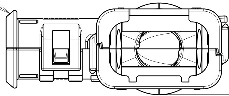
2302491-1 ASSEMBLED VIEW SHOWN DIMENSIONS SHOWN TYPICAL FOR 2302491-1 AND -3
