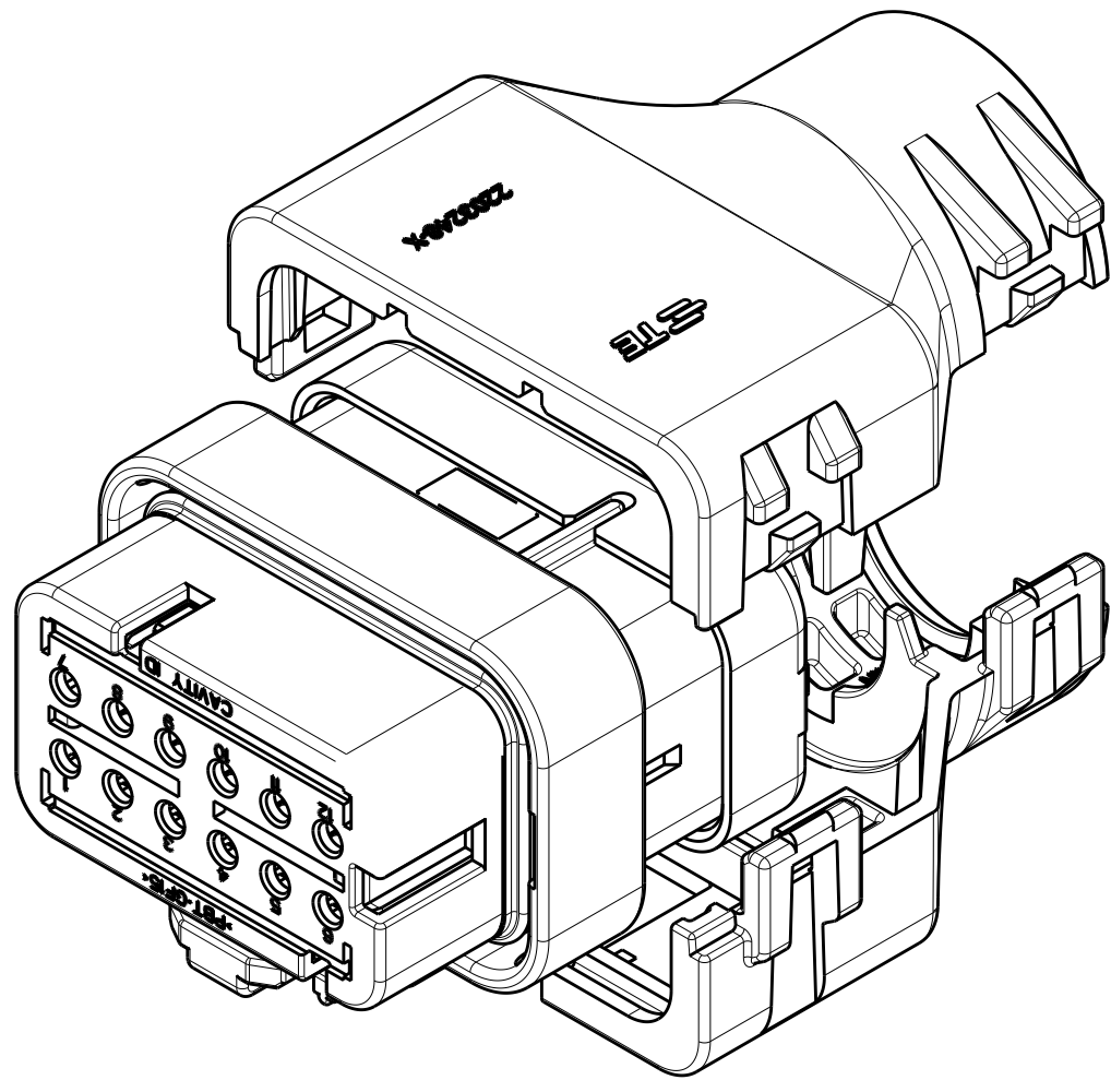
2292802-3 WITH PLUG ASSEMBLY EXPLODED ISOMETRIC VIEW SHOWN
