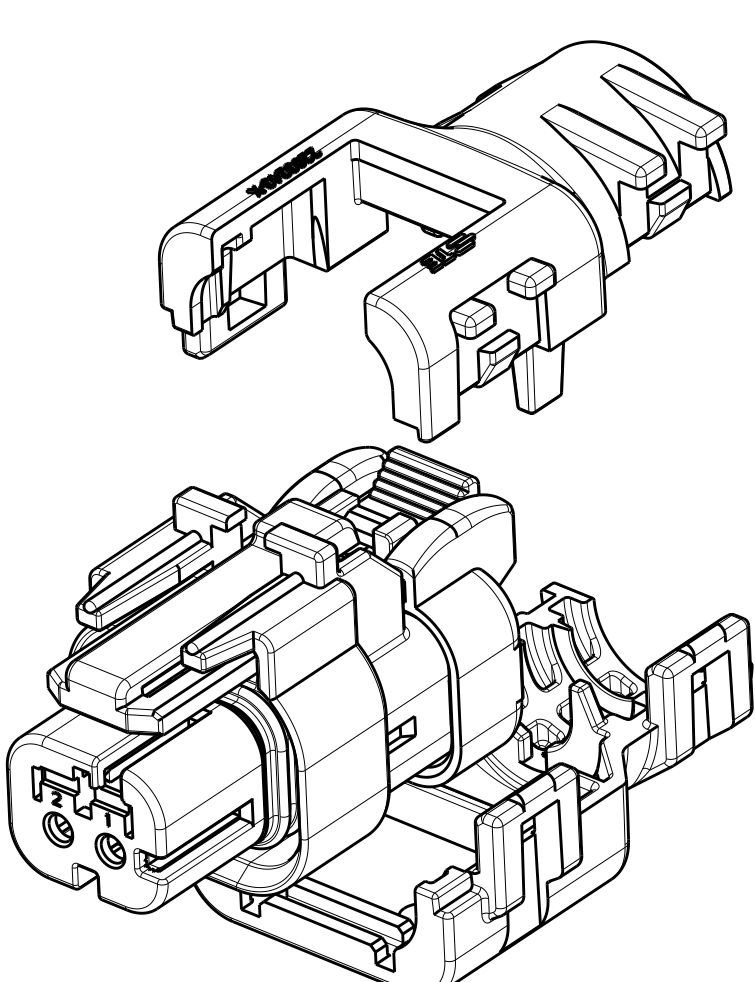
2292797-3 WITH PLUG ASSEMBLY EXPLODED ISOMETRIC VIEW SHOWN
