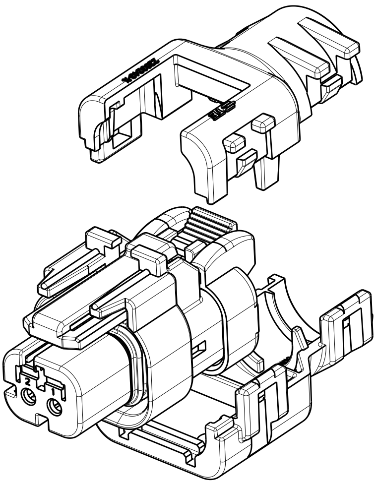
2292797-2 WITH PLUG ASSEMBLY EXPLODED ISOMETRIC VIEW SHOWN
