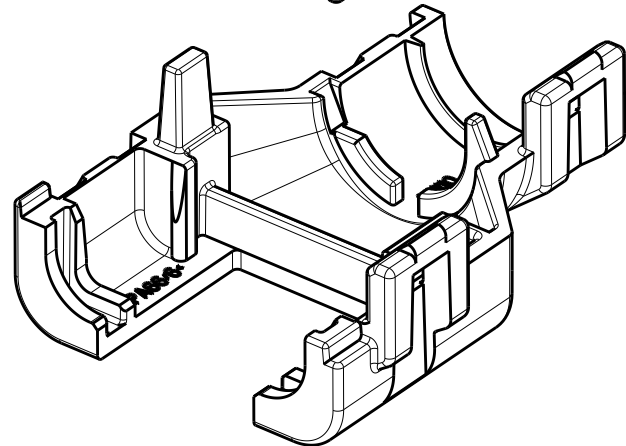
2292798-2 EXPLODED ISOMETRIC VIEW SHOWN
