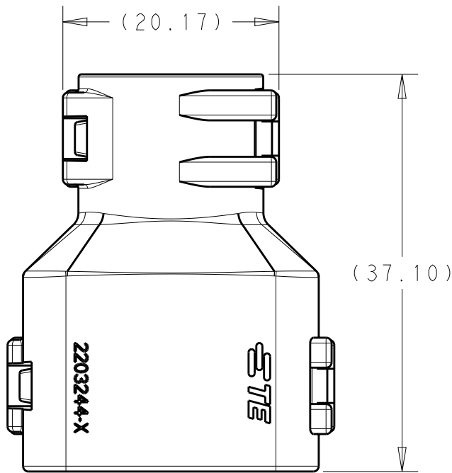
2292798-2 ASSEMBLED VIEW SHOWN
