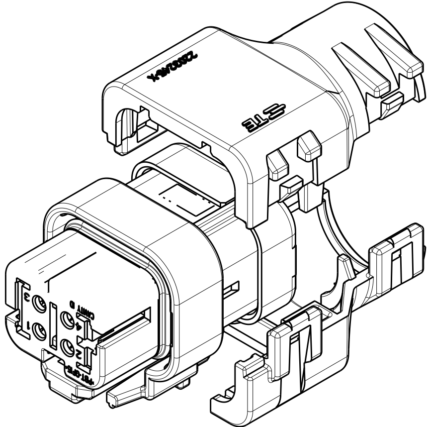
2292799-2 WITH PLUG ASSEMBLY EXPLODED ISOMETRIC VIEW SHOWN
