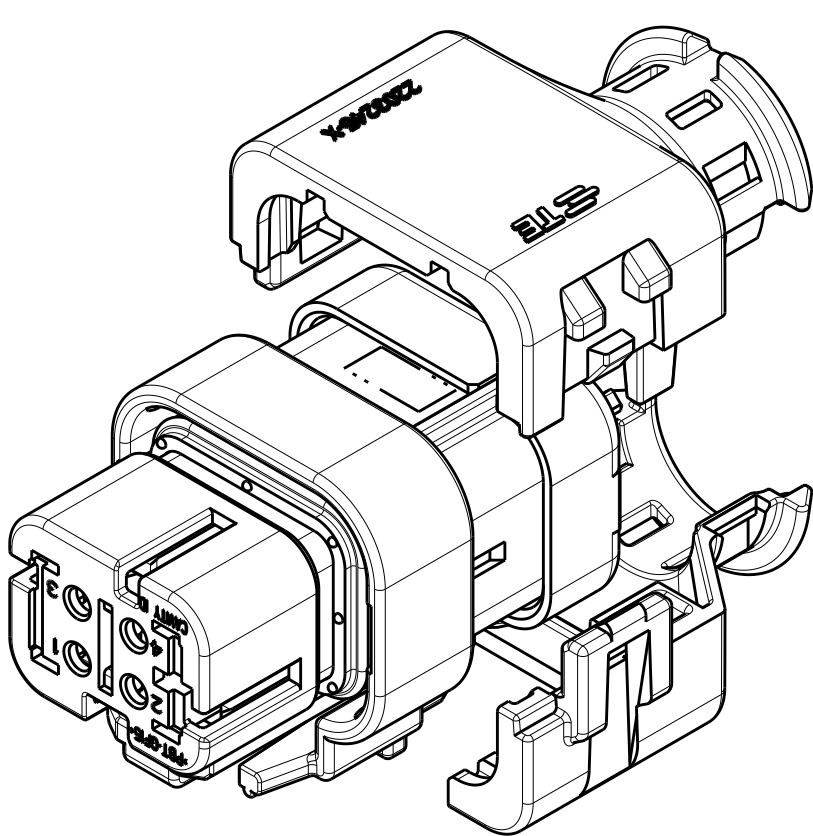
2292799-1 WITH PLUG ASSEMBLY EXPLODED ISOMETRIC VIEW SHOWN
