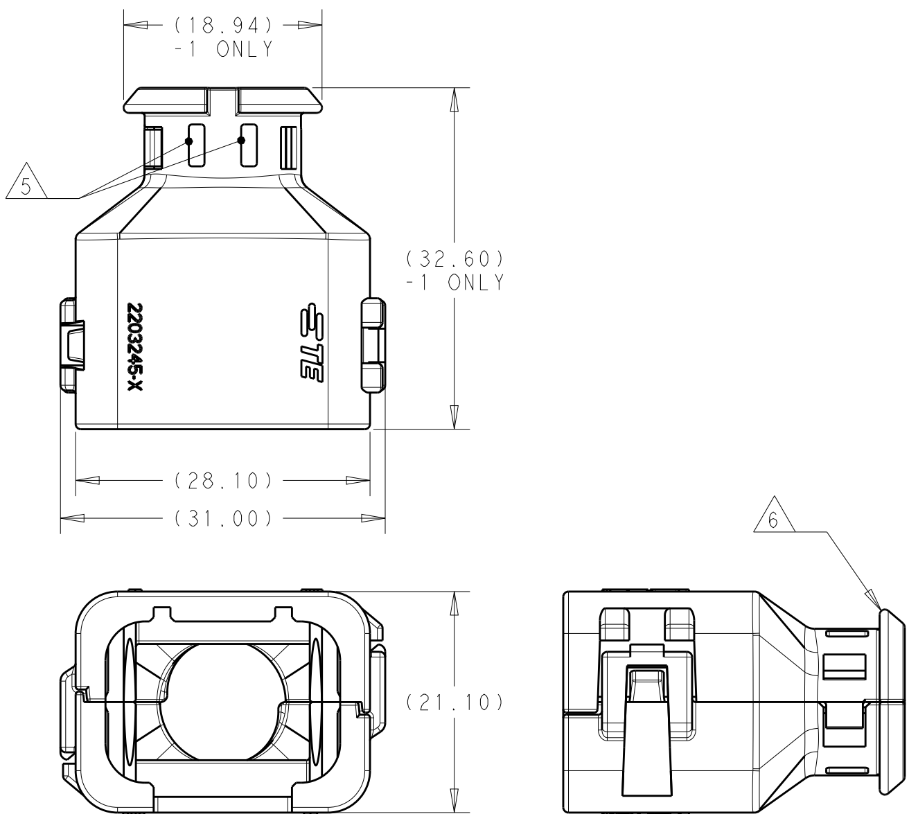
2292799-1 ASSEMBLED VIEW SHOWN
