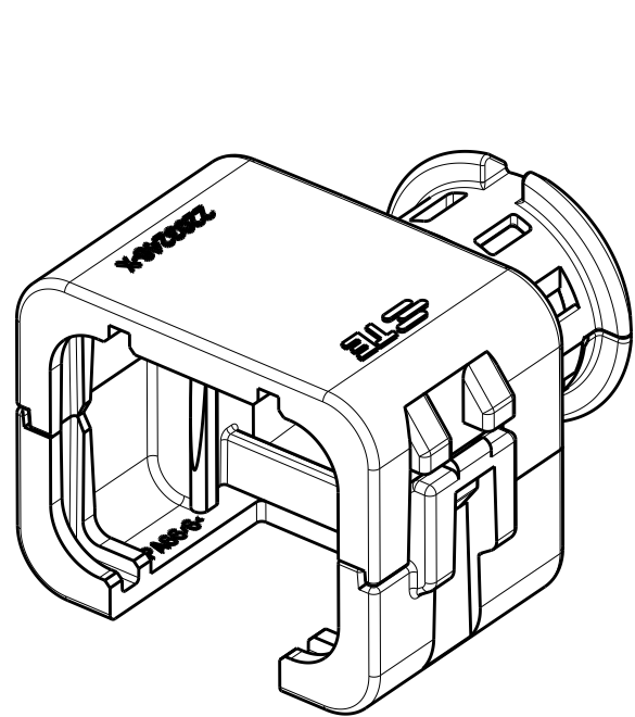
2292800-1 ASSEMBLED ISOMETRIC VIEW SHOWN
