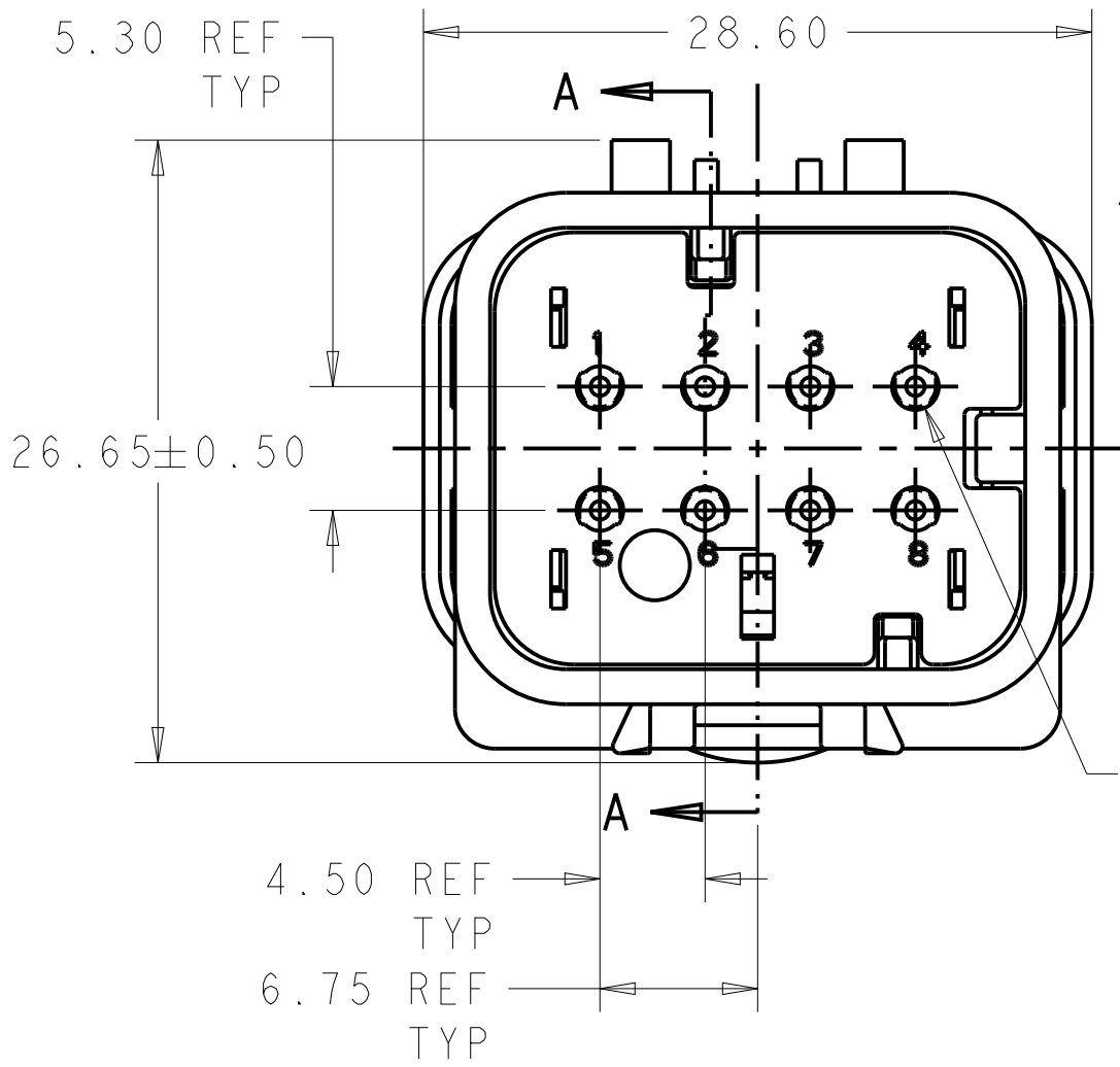
2320930-1 SHOWN KEY A
