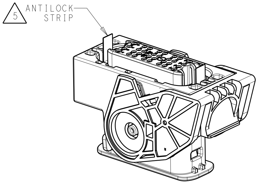
TPA SHOWN IN PRE-MOUNTED POSITION AS RECEIVED
